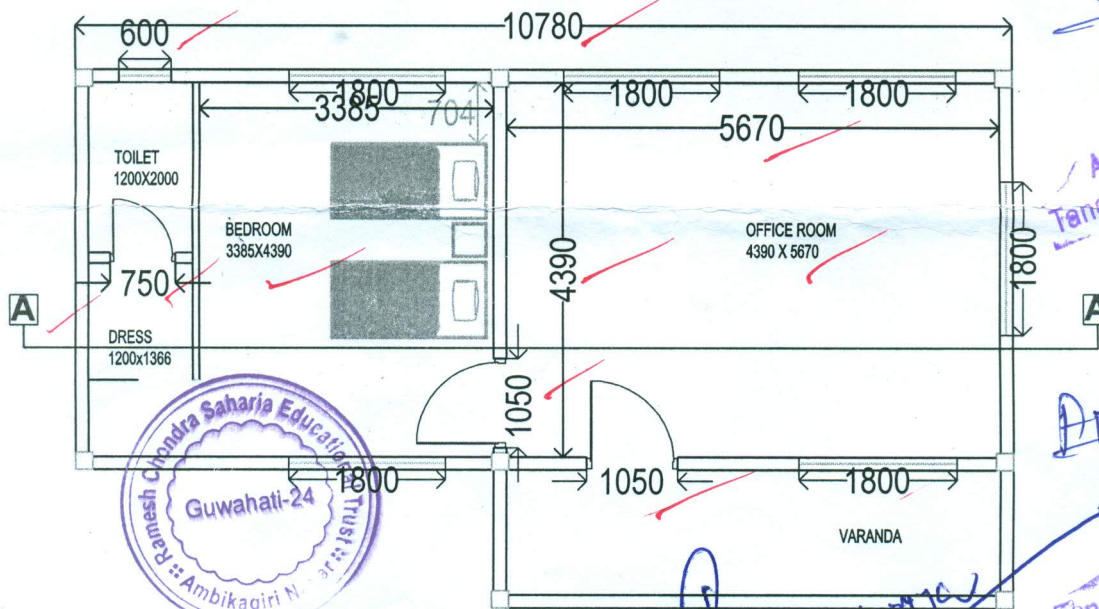
• FLOOR PLAN
